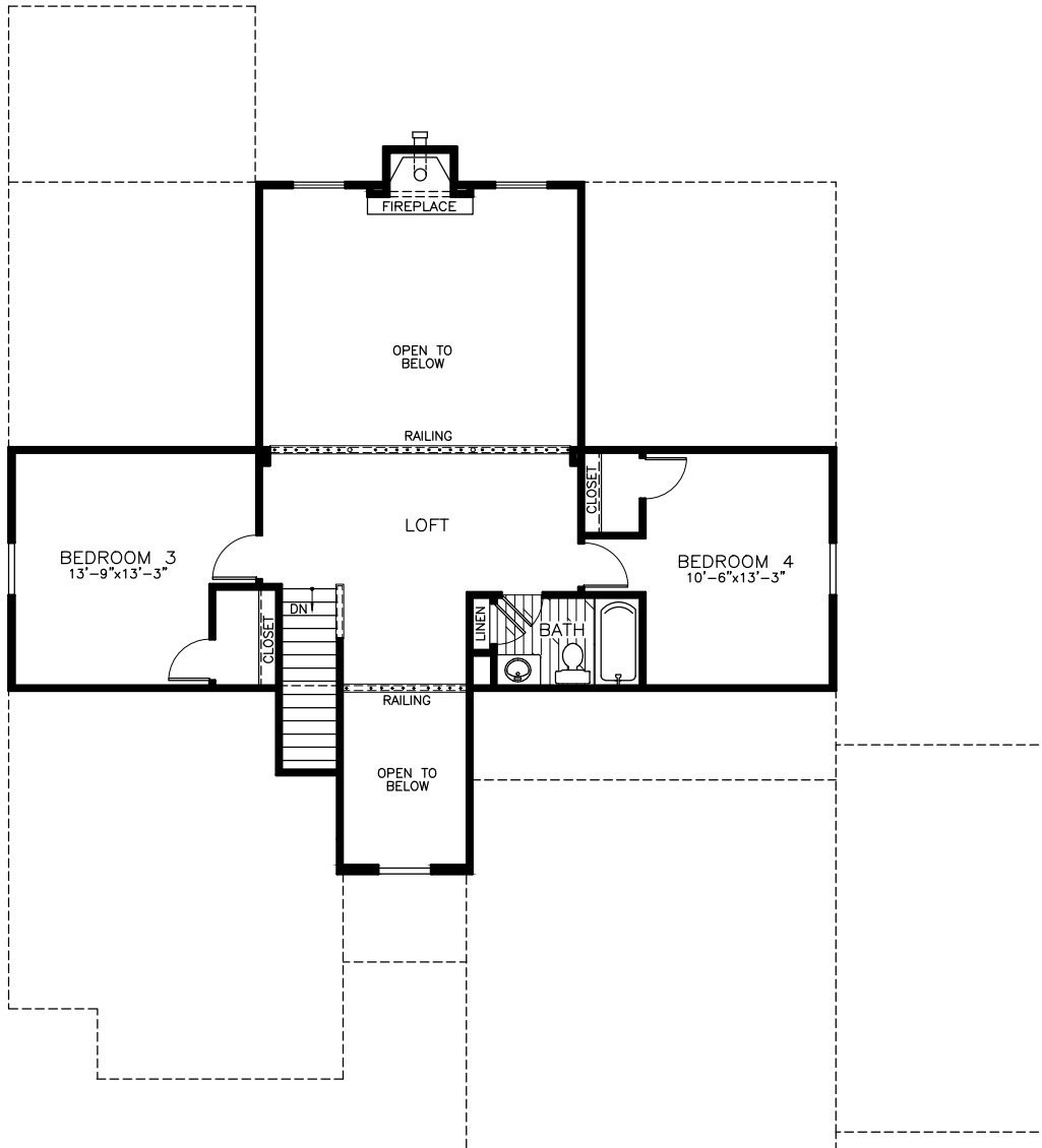
Standard Second Floor Standard Floor Plans 2712 sq. ft.
