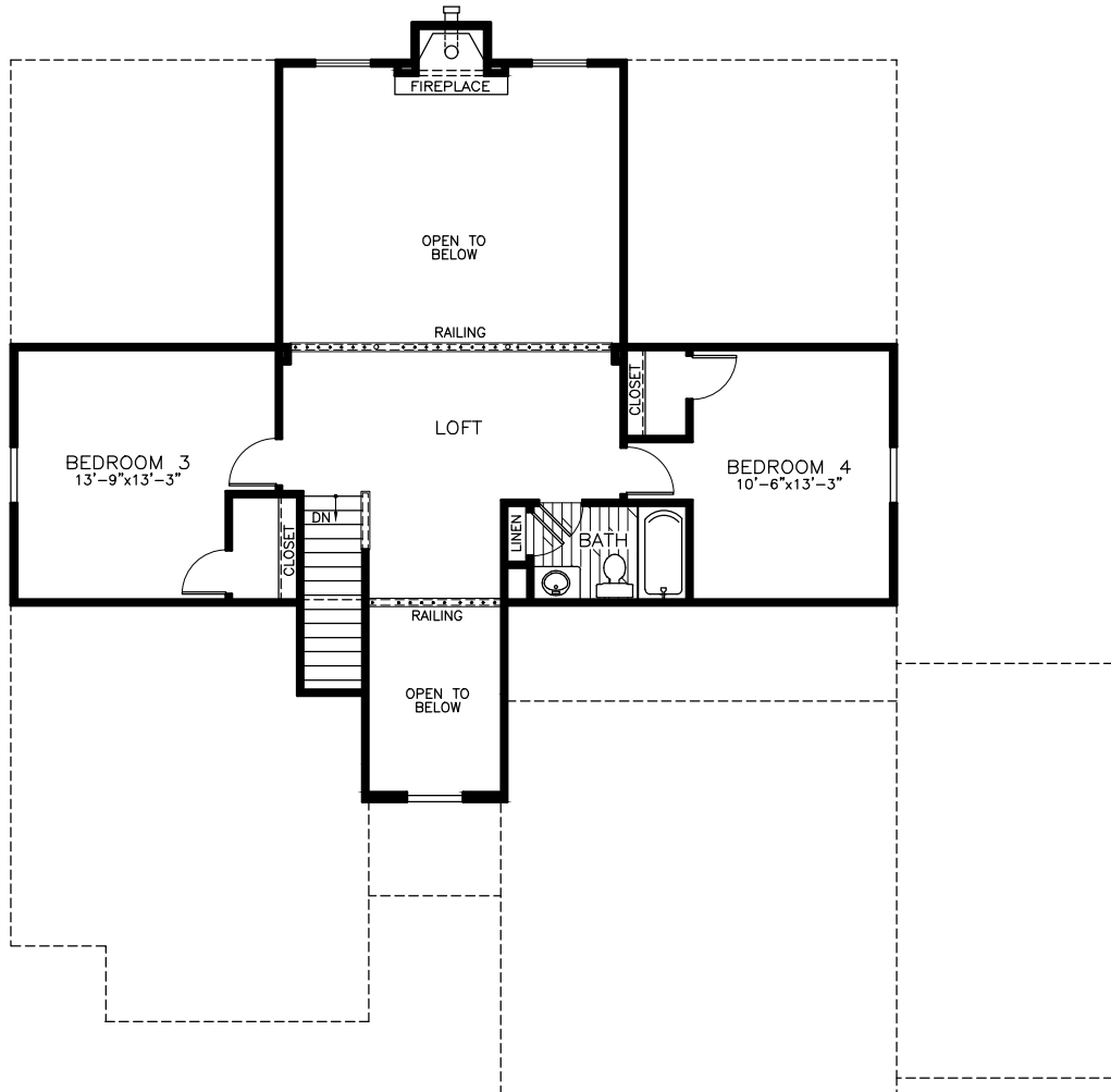
Standard Second Floor Standard Floor Plans 2577 sq. ft.
