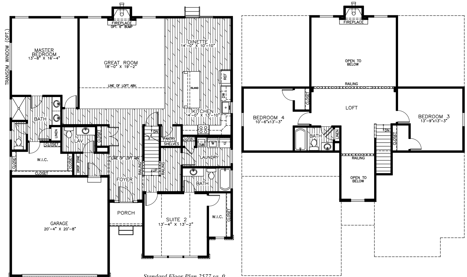
Standard Floor Plan 2577 sq. ft.
