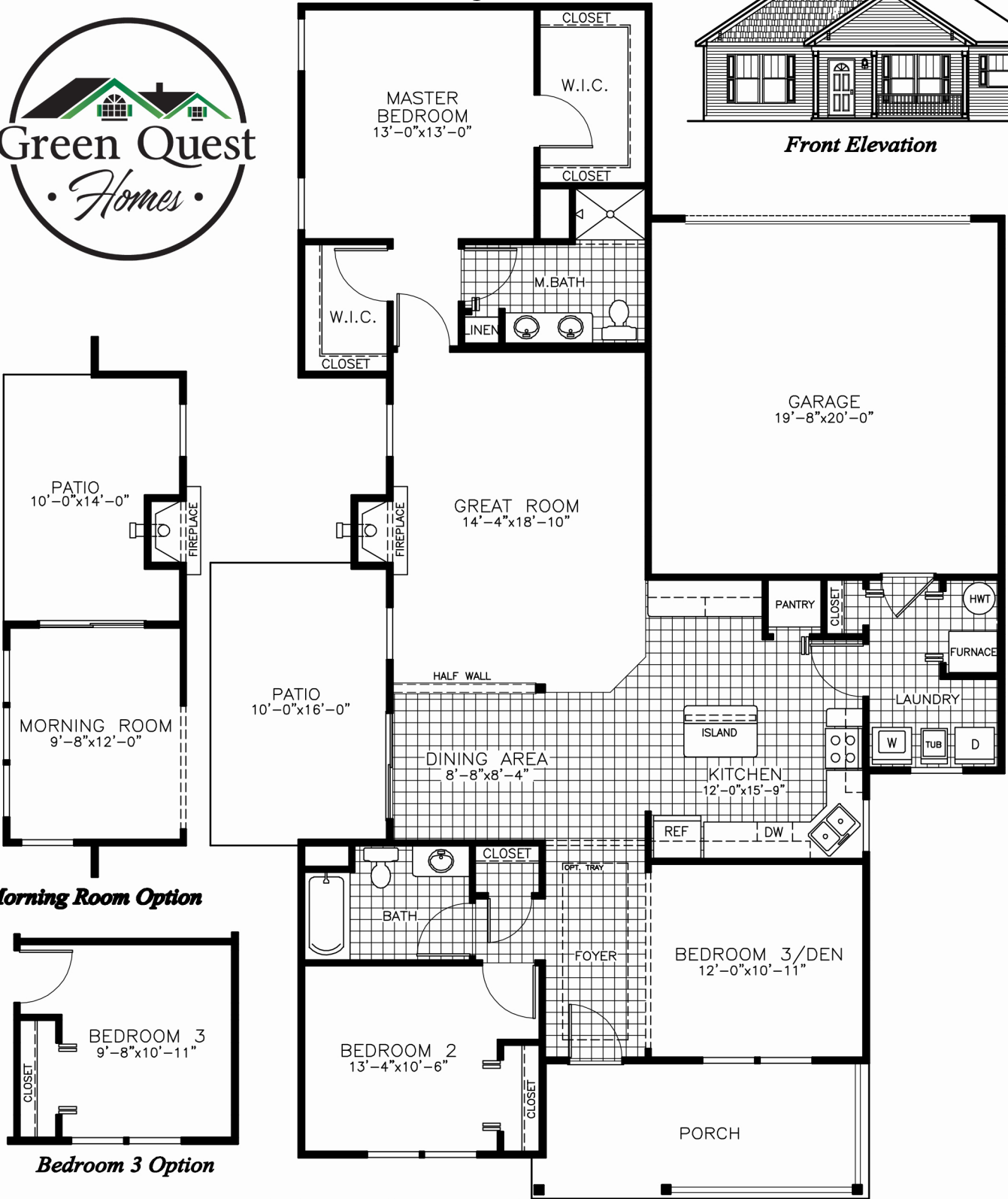
Standard Floor Plan 1570 sq. ft.
