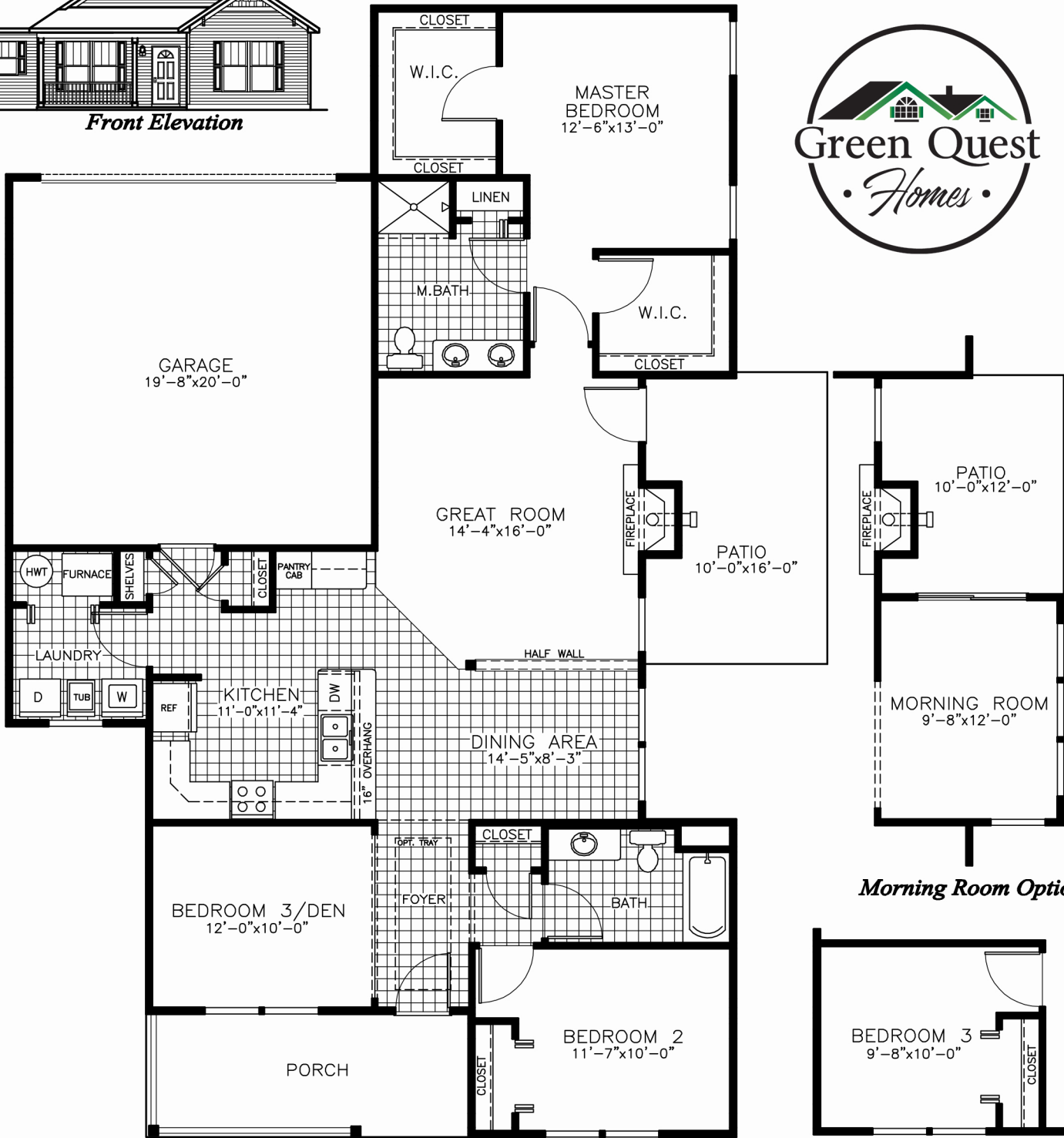
Standard Floor Plan 1475 sq. ft.
